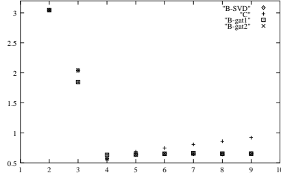
(e) Residuals from the true function
