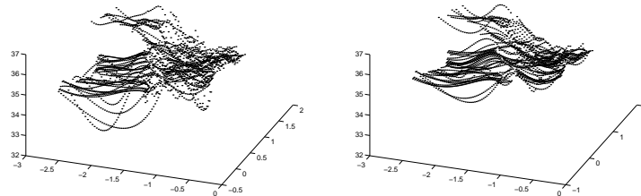
(f) 4th order Chi
