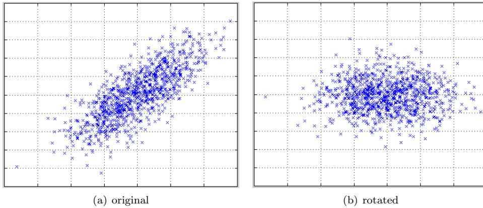
Figure 7: original and rotated data distributions
