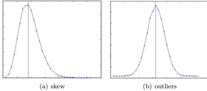
Figure 6: data distributions featuring skew and outliers
