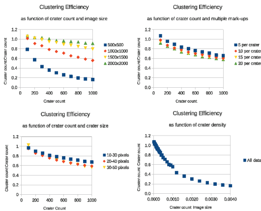
Figure 2: Efficiency of correct clustering
