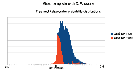
Figure 3: True and false annotation distributions
