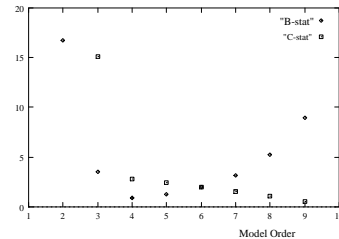
(d) Behaviour of B and Chi Statistics
