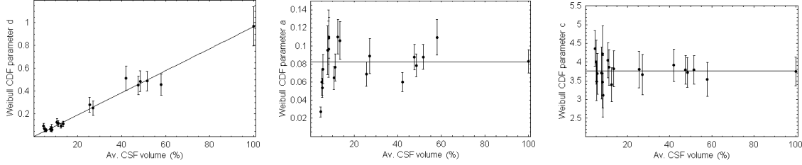
Figure 3. The Weibull fit parameters d , a , and c for all volumes and sub-volumes. Errors were estimated from the confidence interval on the fits themselves, and so are correlated across the parameters.
