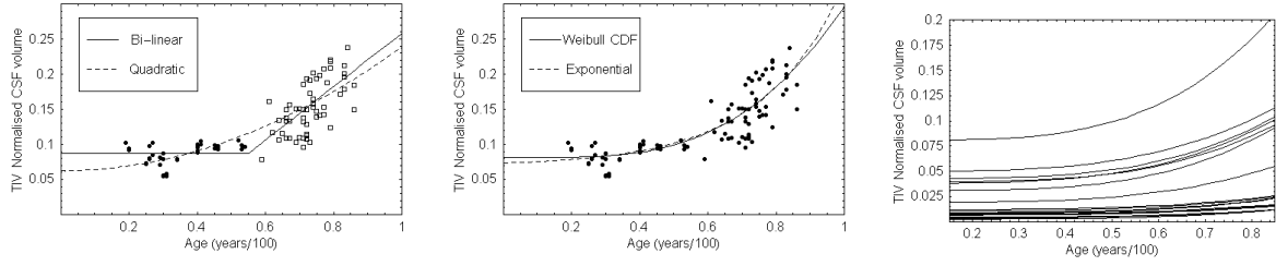
Figure 2. Bi-linear, quadratic, exponential and Weibull CDF fits to the normalised CSF volumes, and Weibull fits to all volumes and sub-volumes (right).
