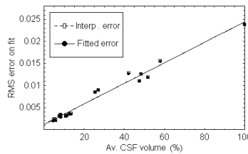
Figure 4. RMS error on fitted and interpolated Weibull CDFs for all sub-volumes.
